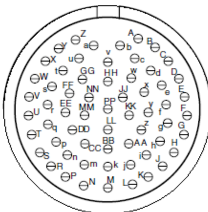
Outside View (Mating Connector)
